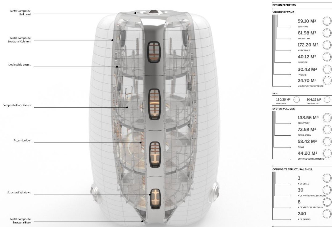
Figure 9. Habitat System Calculations. Axonometric
